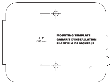
Figure 1: Use Mounting Template (included)
