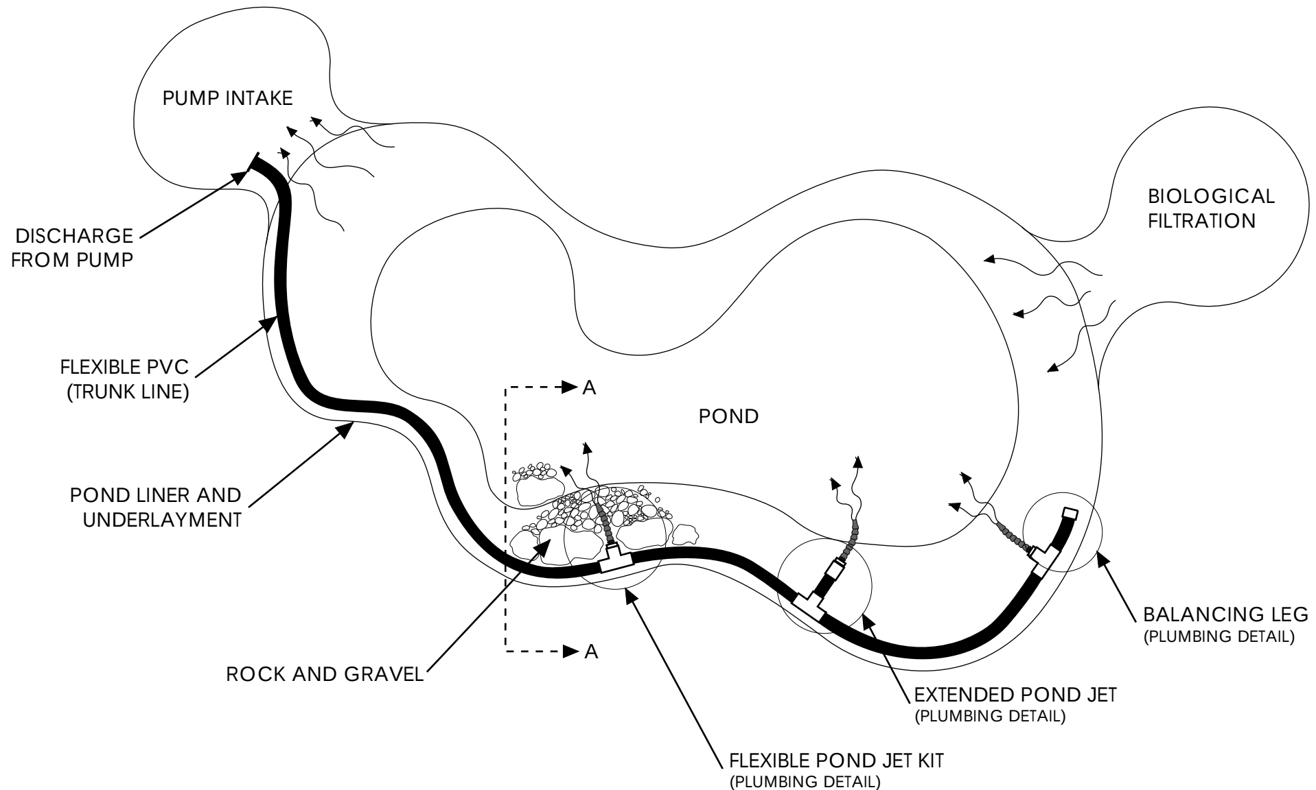
PLAN VIEW
